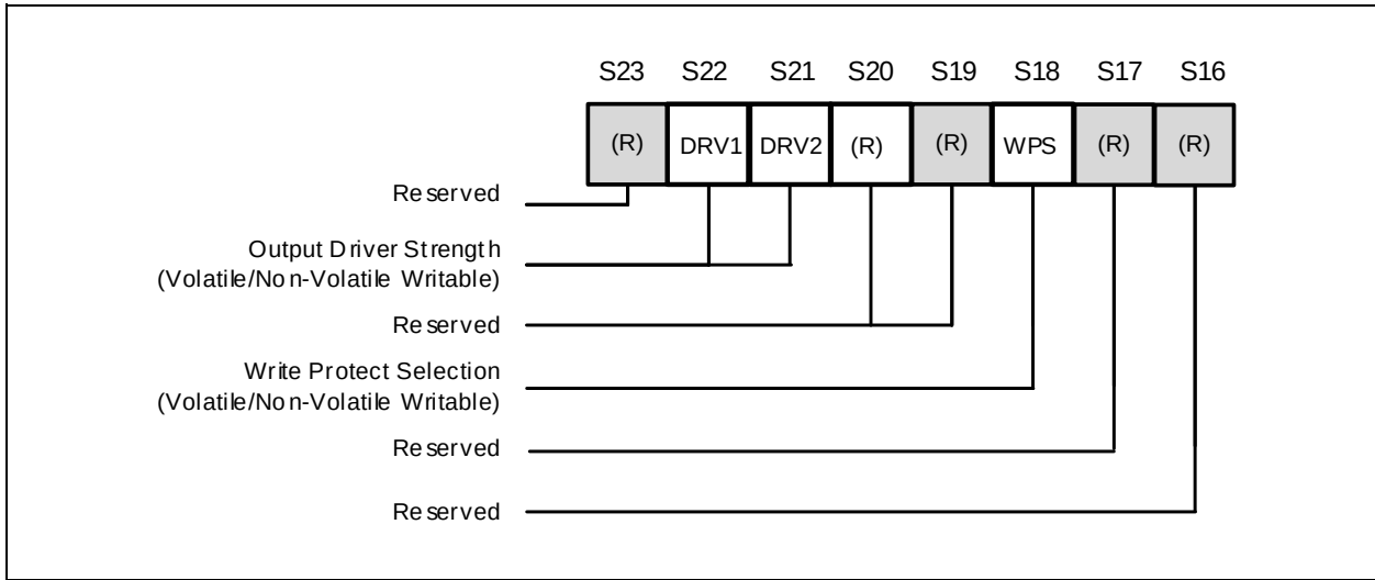
Figure 3c. Status Register-3
